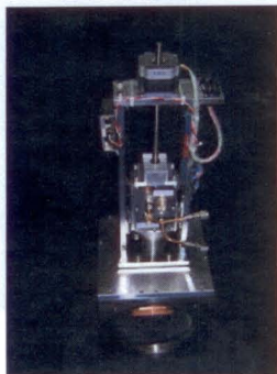
Emittance Scanner**
